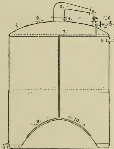
FIG. 98.—Vertical Still for Refining Coal Tar.
